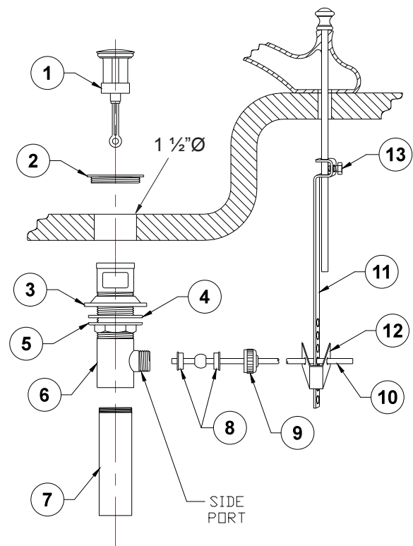
COMPONENT PARTS
