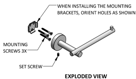
EXPLODED VIEW
