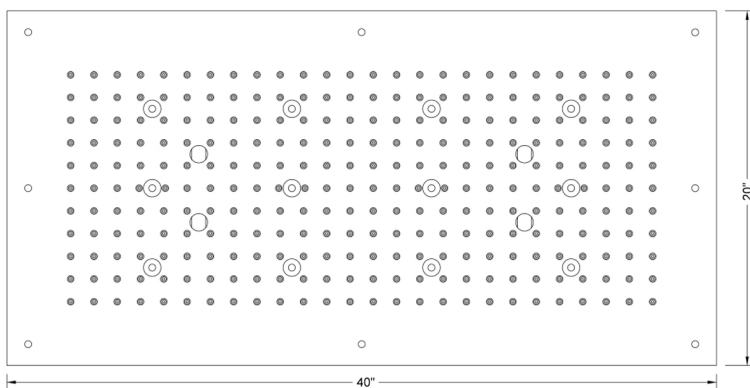
BOTTOM VIEW
